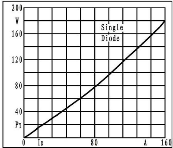
Fig2. Power dissipation
